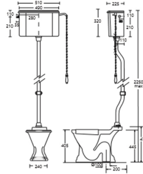
Birmingham Toilet S trap with High Level Cistern
